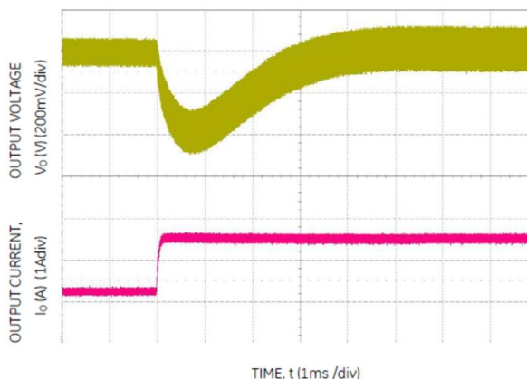
Figure 10. Transient Response to Dynamic Load Change from 50% to 100% at 12Vin, C_{out}=3\times 10\mu\text{F}+220\mu\text{F} , C_{Tune}=3300\text{pF} , R_{Tune}=30.1\text{k}\Omega
