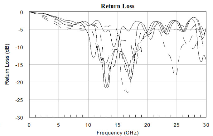
Typical Performance 12.0 to 19.0 GHz
