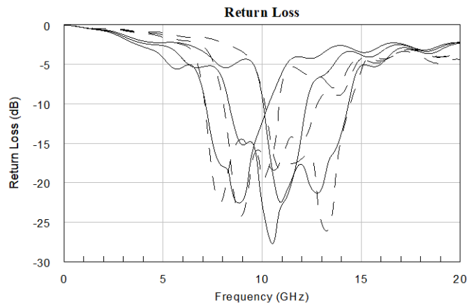
Typical Performance 8.0 to 13.5 GHz
