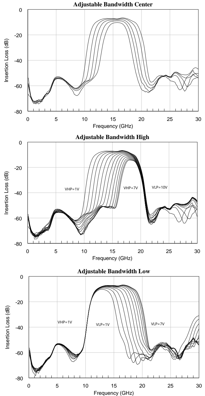
Typical Performance 12.0 to 19.0 GHz
