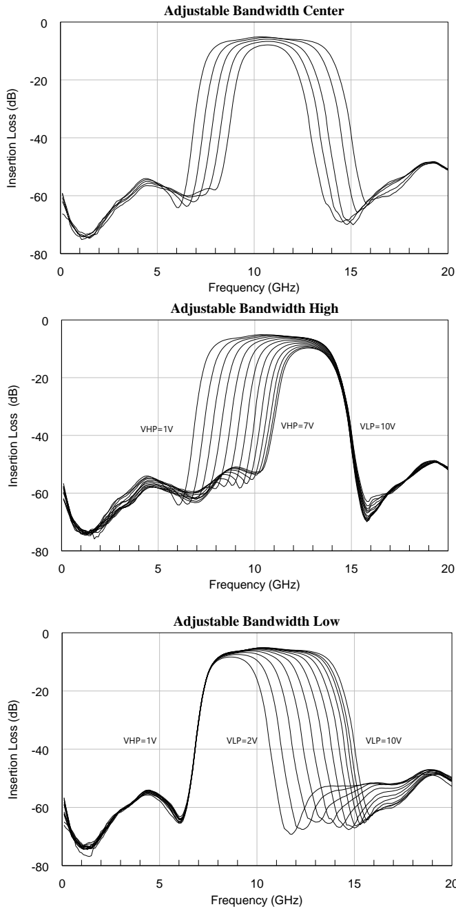
Typical Performance 8.0 to 13.5 GHz
