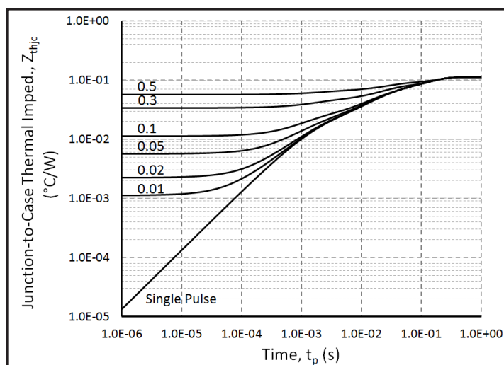
Figure 17. FET Junction to Case Transient Thermal Impedance, Z_{thJC} \text{ (}^\circ\text{C/W)}
