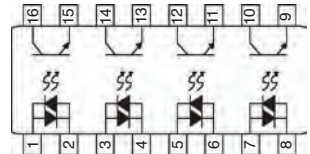
Darlington Output
