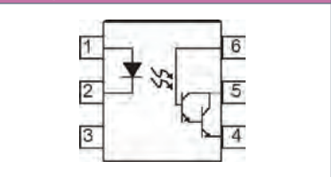
Darlington Output - High Voltage
