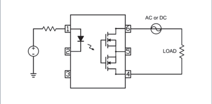
Output Configuration A
