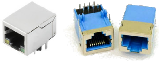
Side Entry
