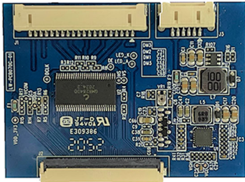
LVDS to RGB with LED driver
