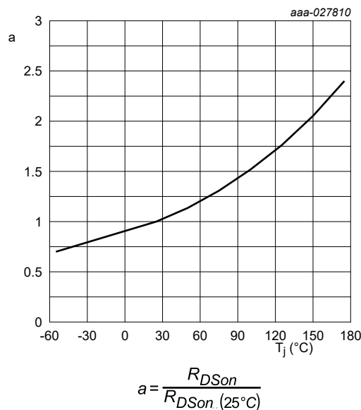
Fig. 2. Normalized drain-source on-state resistance factor as a function of junction temperature
