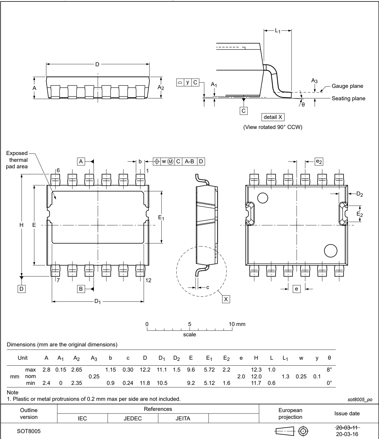
Fig. 5. Package outline CCPAK (SOT8005)
