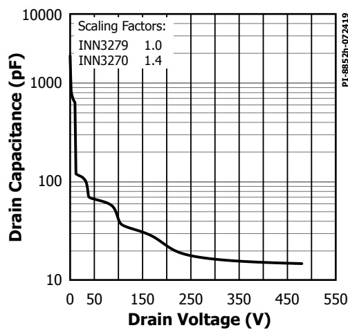
Figure 36. C_{OSS} vs. Drain Voltage.
