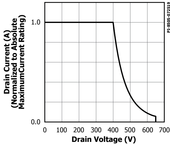
Figure 24. Maximum Allowable Drain Current vs. Drain Voltage (INN326x).
