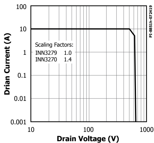
Figure 38. Maximum Allowable Drain Current vs. Drain Voltage (GaN-based INN3279/70).
