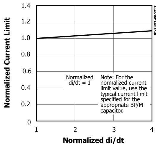
Figure 34. Standard Current Limit vs. di/dt .
