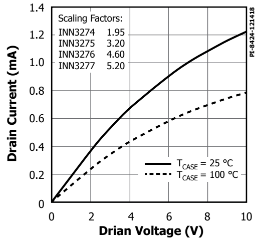
Figure 31. Output Characteristics.
