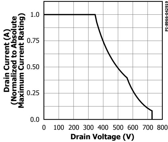
Figure 30. Maximum Allowable Drain Current vs. Drain Voltage (INN3274/75/76/77).
