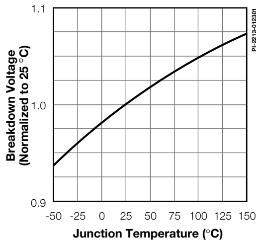
Figure 28. Breakdown vs. Temperature (Exclude INN3279C/INN3270C).
