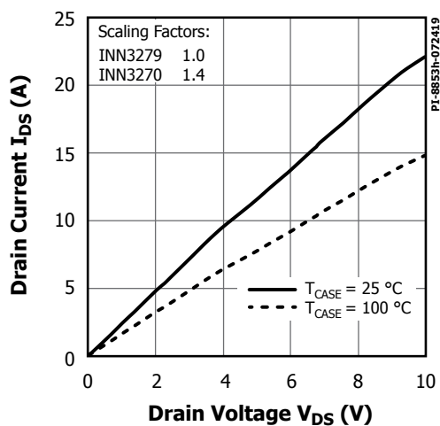
Figure 35. Output Characteristics.
