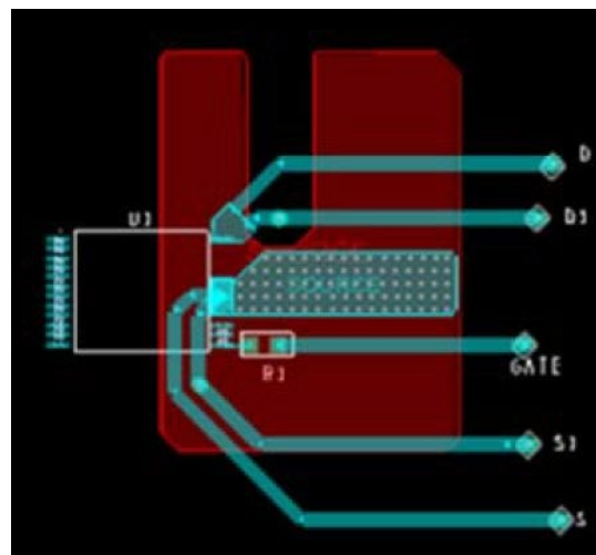
Figure 23. Thermal Resistance Test Conditions for GaN-based INN3279C and INN3270C.
